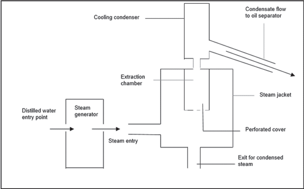
Fig. S1. Diagram of the steam distillation apparatus
