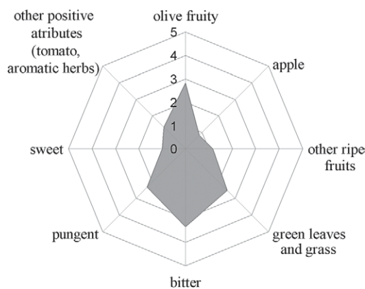
Fig. 2. Sensory profile of Bova cultivar virgin olive oil. Results are mean values of 3 independent repetitions (median of eight assessments for each descriptor). Numbers 0–5 represent perception intensity of sensory characteristics: 0=no perception, 1=scarce, 2=light, 3=medium, 4=strong, 5=extreme
