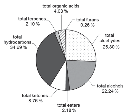
Fig. 3. The amounts of volatile compounds (percentage of total peak area) in Bova cultivar virgin olive oil. Results are expressed as mean values of peak area of three independent repetitions
