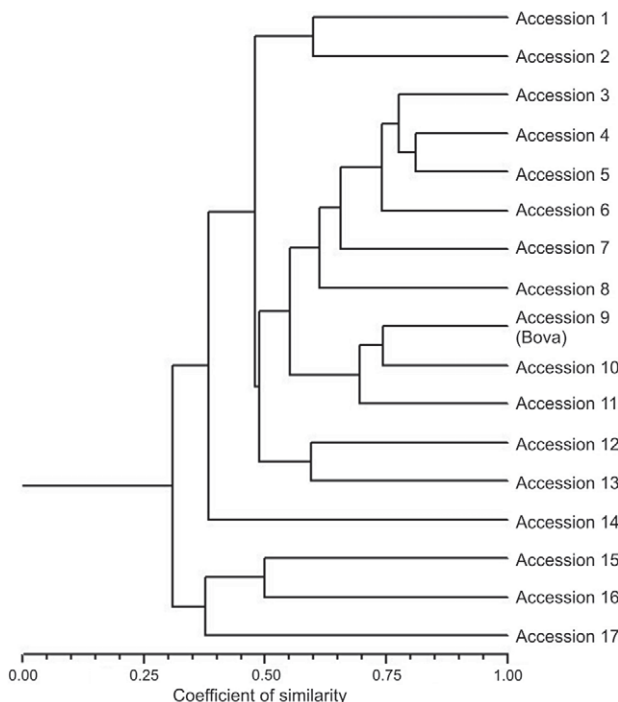
Fig. 1. Dendrogram of 17 Istrian accessions based on Lynch's genetic similarity index data
