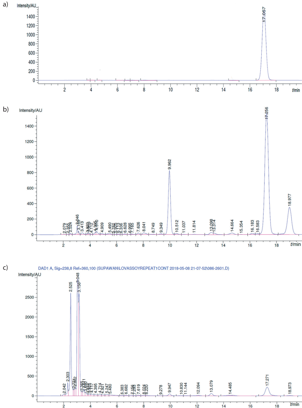
Fig. S1. HPLC chromatograms of: a) lovastatin standard, and crude lovastatin extracts from: b) ethyl acetate and c) hexane
