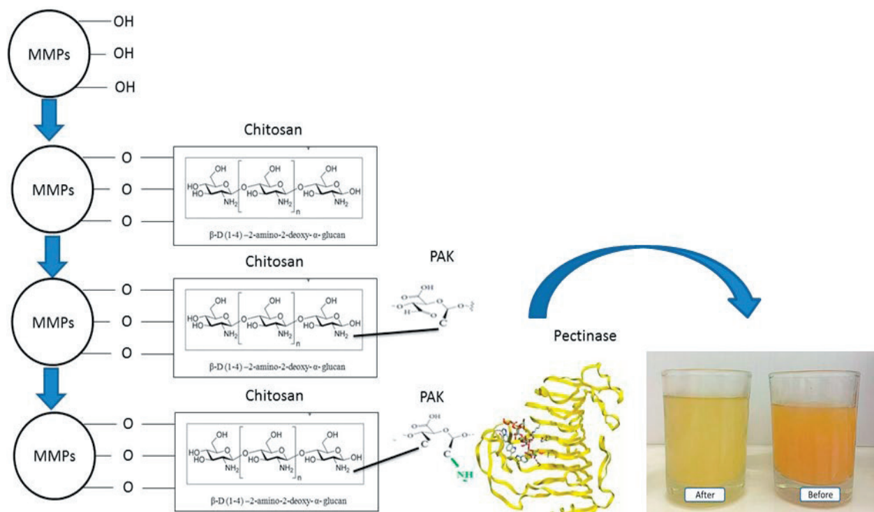
Fig. S1. Scheme of enzyme immobilization steps
