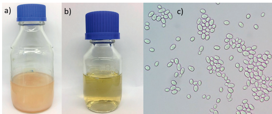
Fig. S1. Cocoa honey: a) before ( A_{600\text{ nm}}=1.165 ) and b) after ( A_{600\text{ nm}}=0.084 ) fermentation by c) S. cerevisiae L63 (observed under a microscope at 400× magnification)
