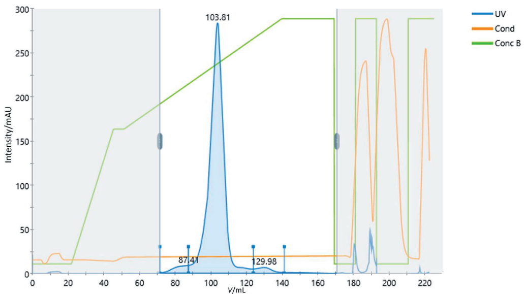
Fig. S2. Chromatogram of the salt-mediated pH elution experiment at pH=5.0–9.1 and c(NaCl)=0–50 mM
