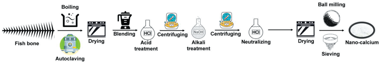
Fig. S1. Production process of nano-calcium powder
