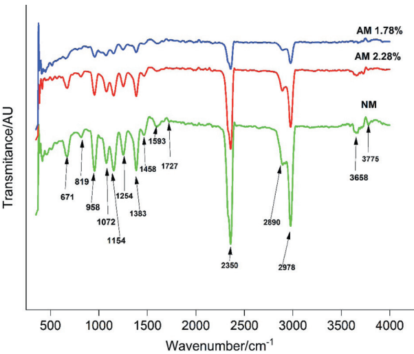
Fig. 1. Spectra of native mucilage (NM), mucilage acetylated to 1.78 % (AM 1.78 %) and mucilage acetylated to 2.28 % (AM 2.28 %) of Opuntia atropes obtained by Fourier transform infrared spectroscopy (FTIR)
